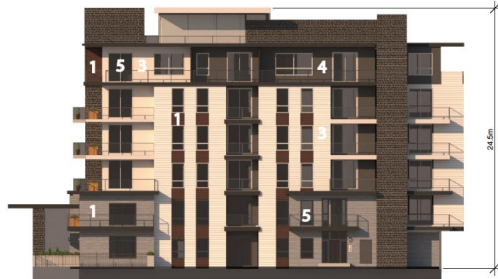
SOUTH ELEVATION
