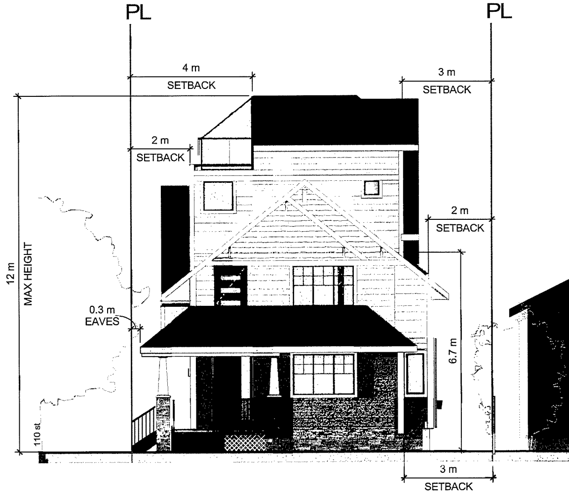
APPENDIX 2c SOUTH ELEVATION
