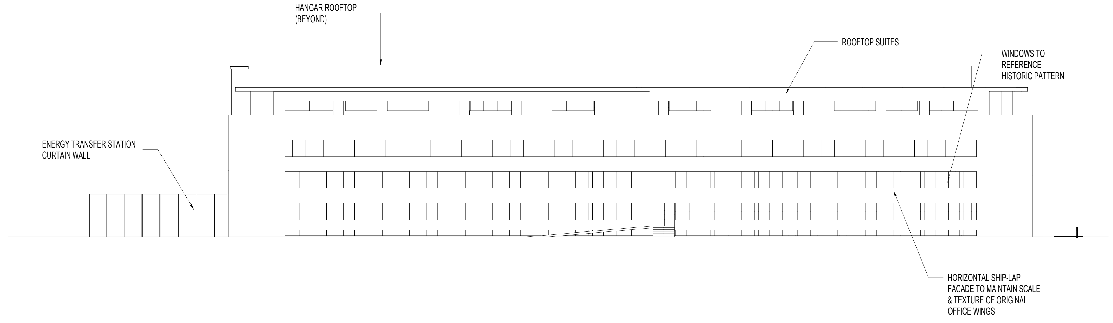
WEST ELEVATION
