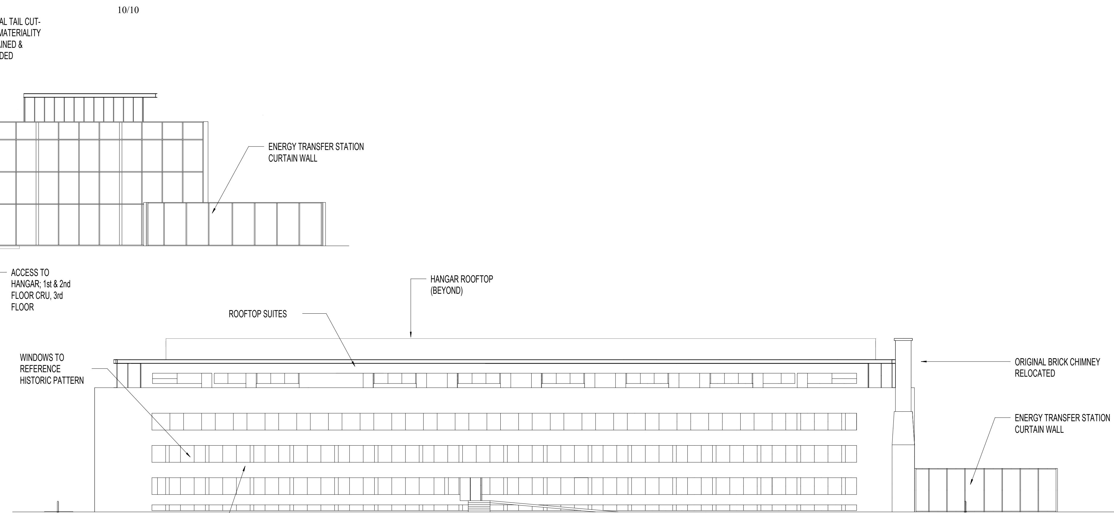
EAST ELEVATION
