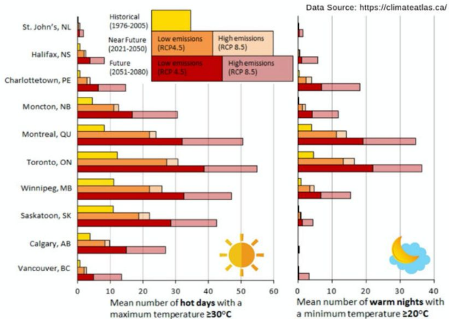
Figure 5: Projected number of hot days and warm nights in select Canadian cities under a changing climate.
