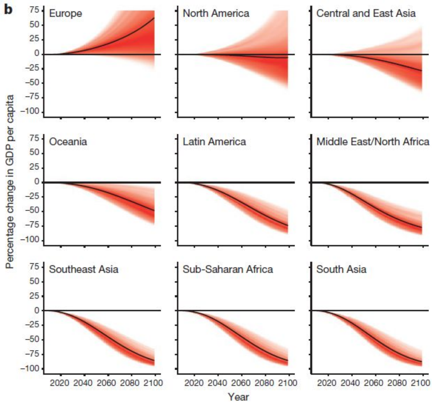
Figure 4 | Projected effect of temperature changes on regional economies. a, b, Change in GDP per capita (RCP8.5, SSP5) relative to projection using constant 1980–2010 average temperatures. a, Country-level estimates in 2100. b, Effects over time for nine regions. Black lines are projections using point estimates. Red shaded area is 95% confidence interval, colour saturation indicates estimated likelihood an income trajectory passes through a value 27 . Base maps by ESRI.
