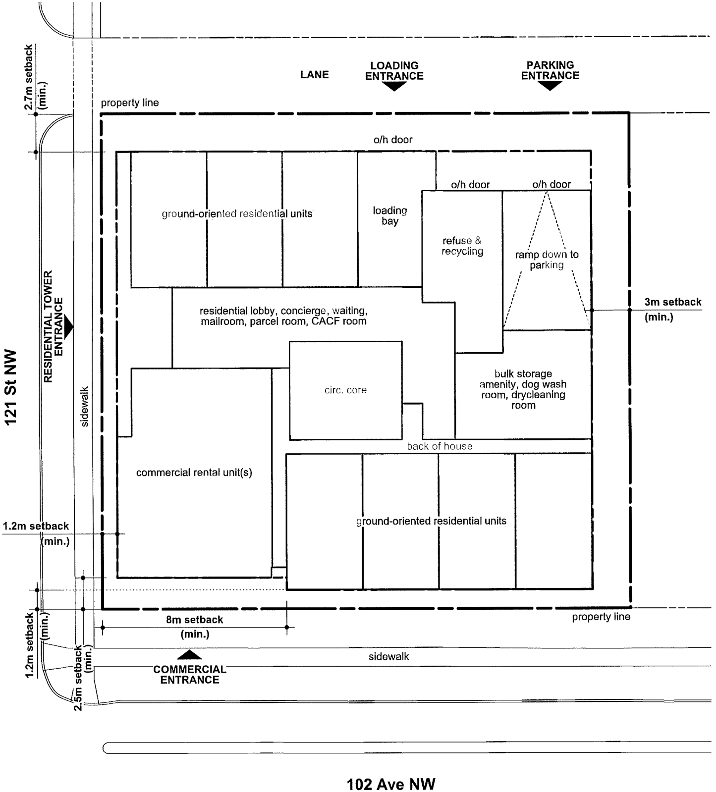
Appendix VI - Conceptual Ground Level Floor Plan (Podium Level 1)
