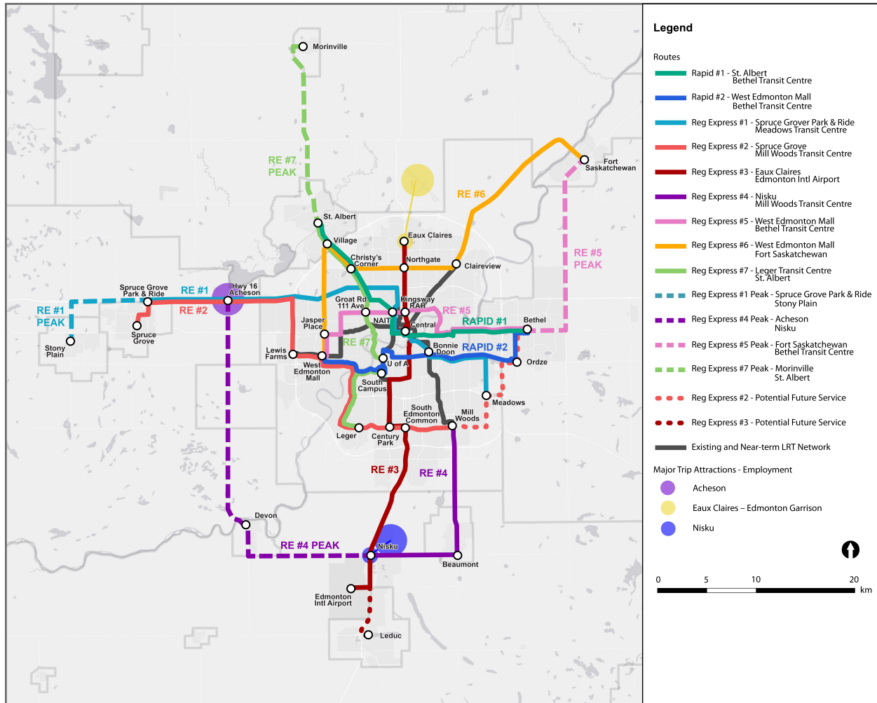
Figure 2 - RTSC conceptual transit services design
