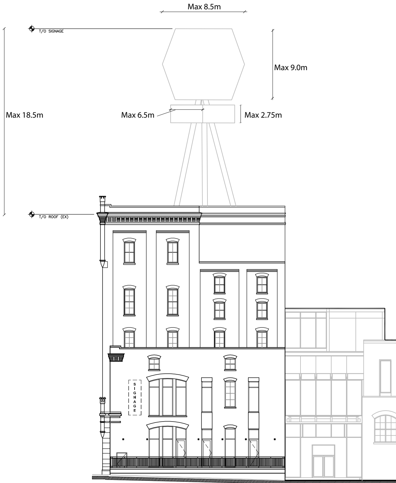
SOUTH ELEVATION
