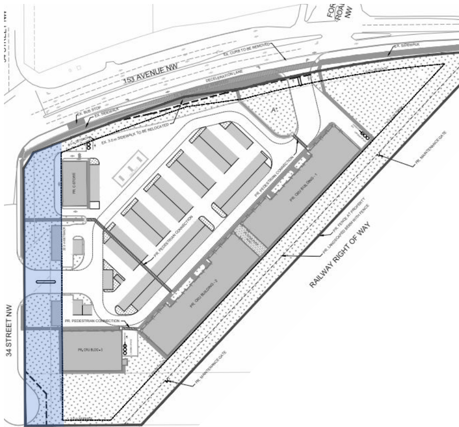
CURRENT/APPROVED SITE PLAN
