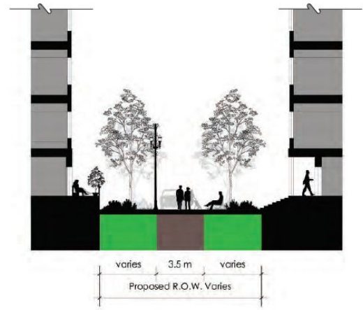
Figure 48: Greenway Section
