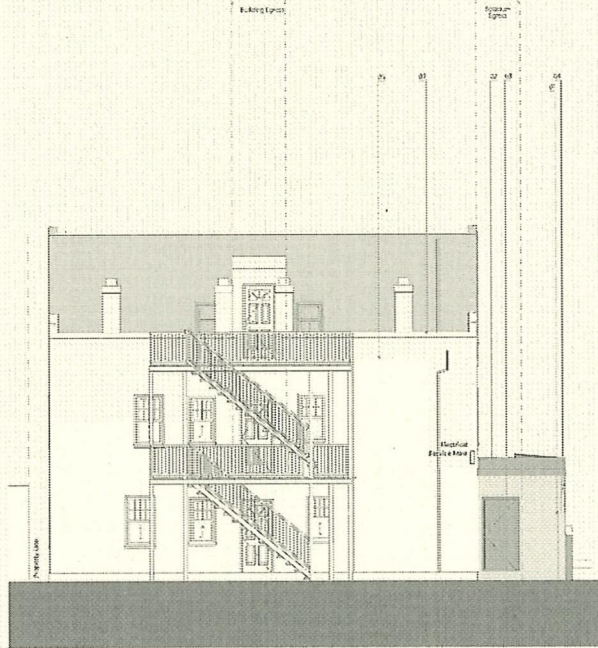
2 A101 East Elevation SCALE: 1/4" = 1'-0"
