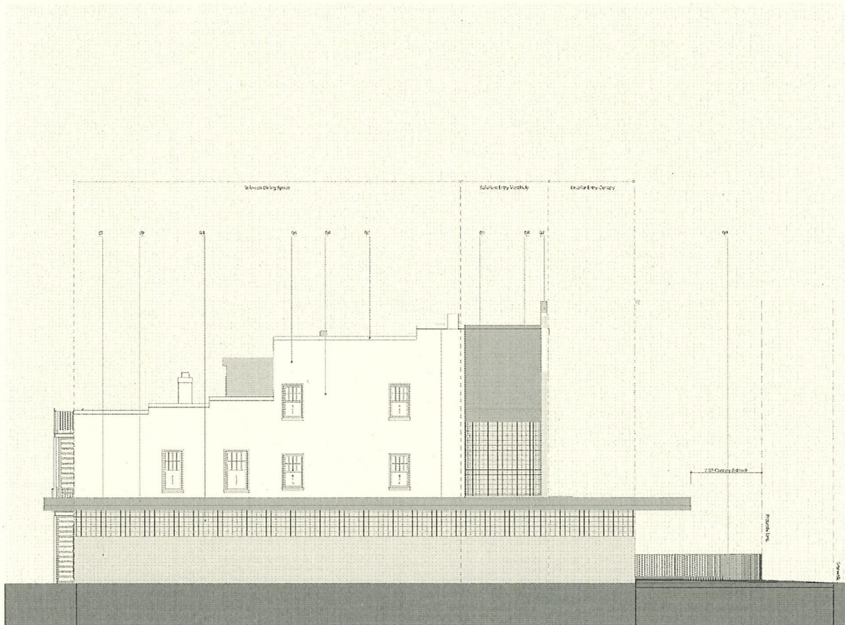
1 North Elevation A102 SCALE: 1/4" = 1'-0"
