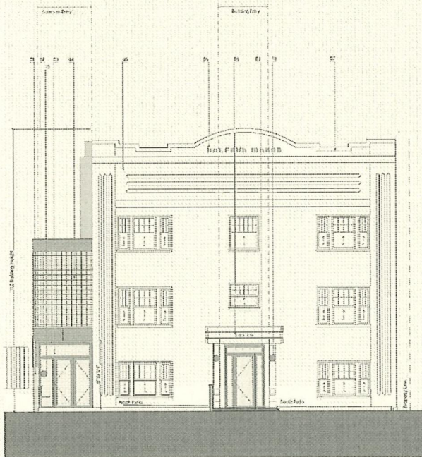
1 A101 West Elevation SCALE: 1/4" = 1'-0"
