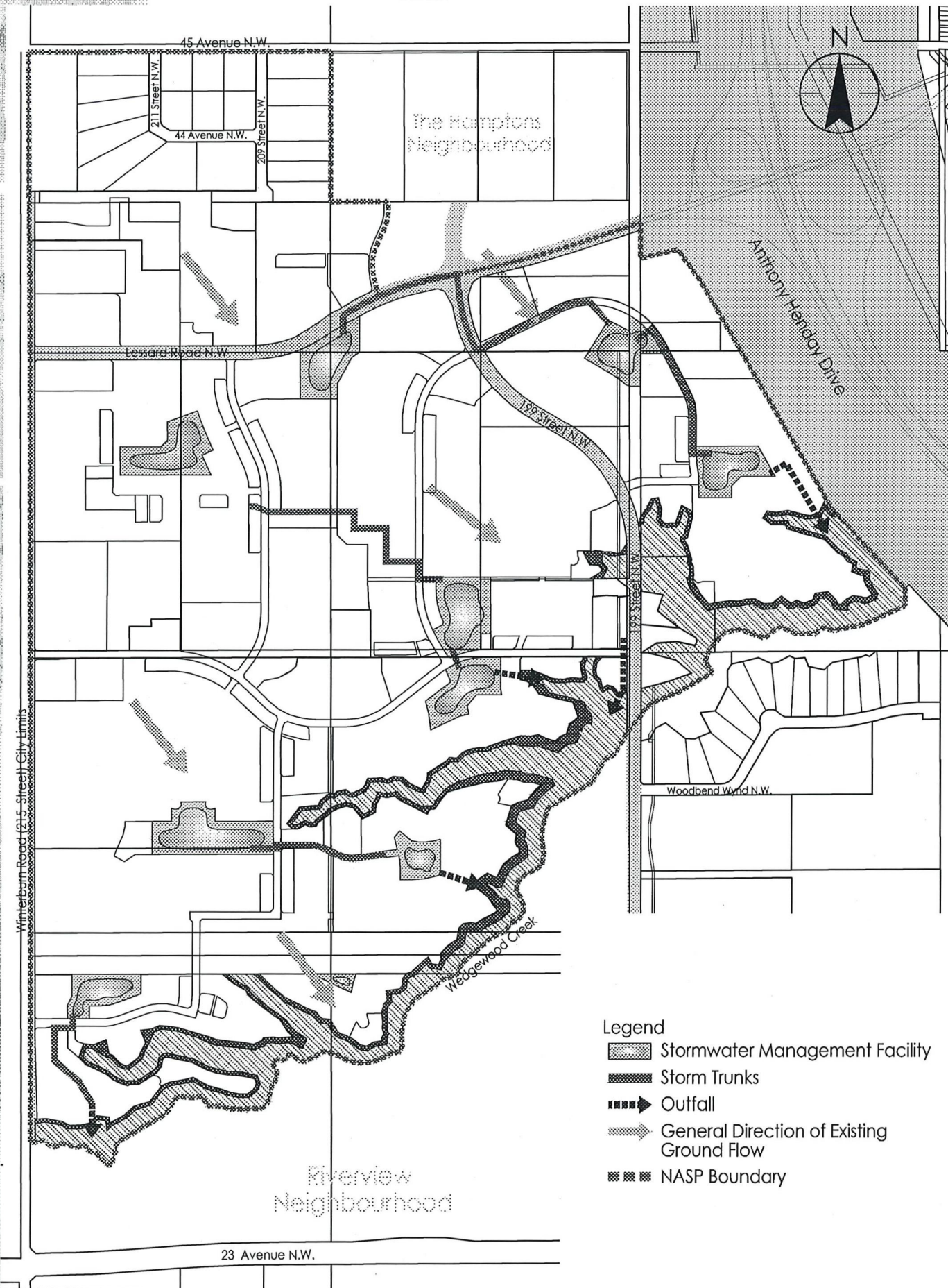
Figure 11 - Stormwater Network Edgemont Neighbourhood Area Structure Plan
