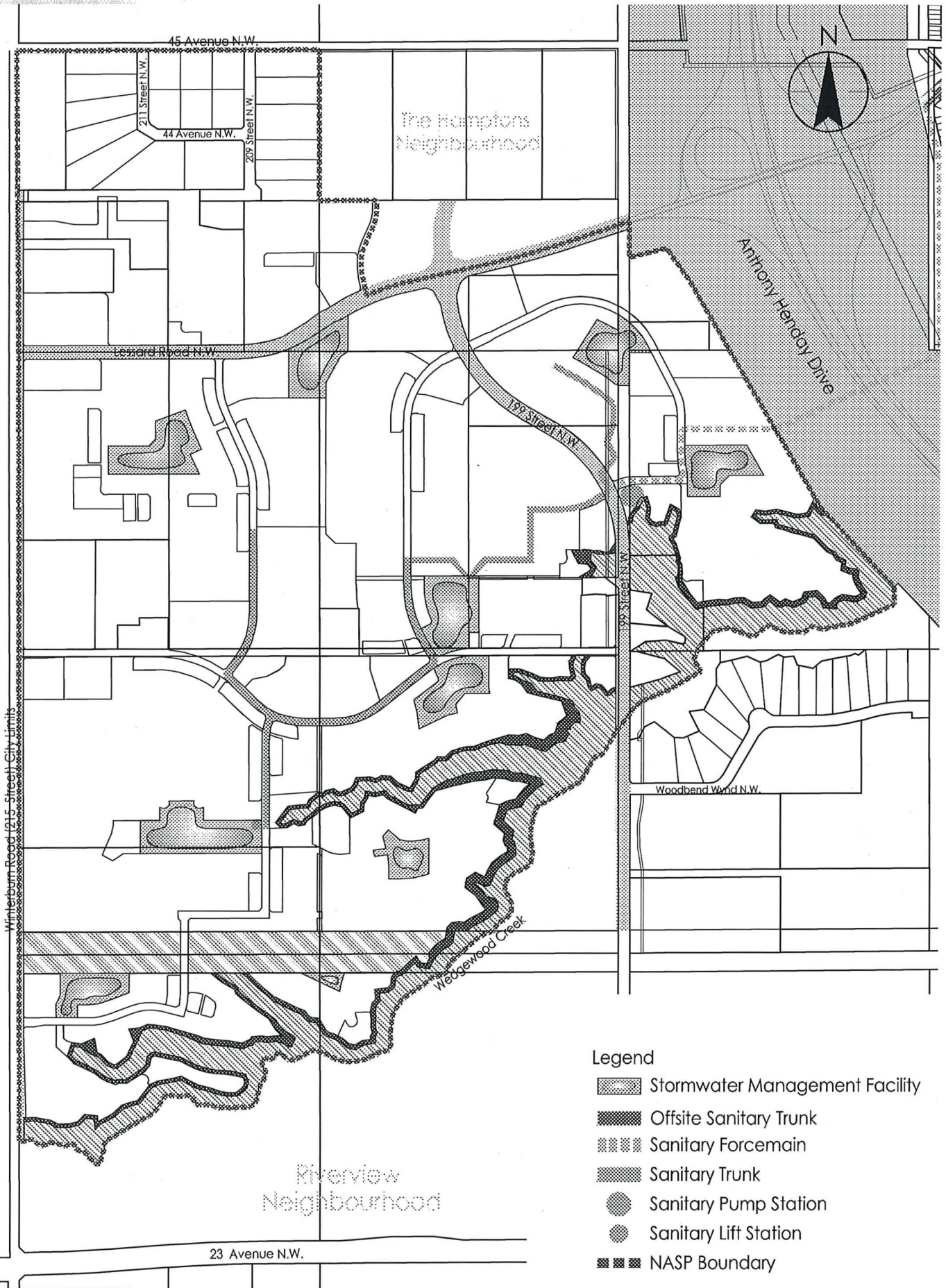
Figure 10 - Sanitary Servicing Edgemont Neighbourhood Area Structure Plan
