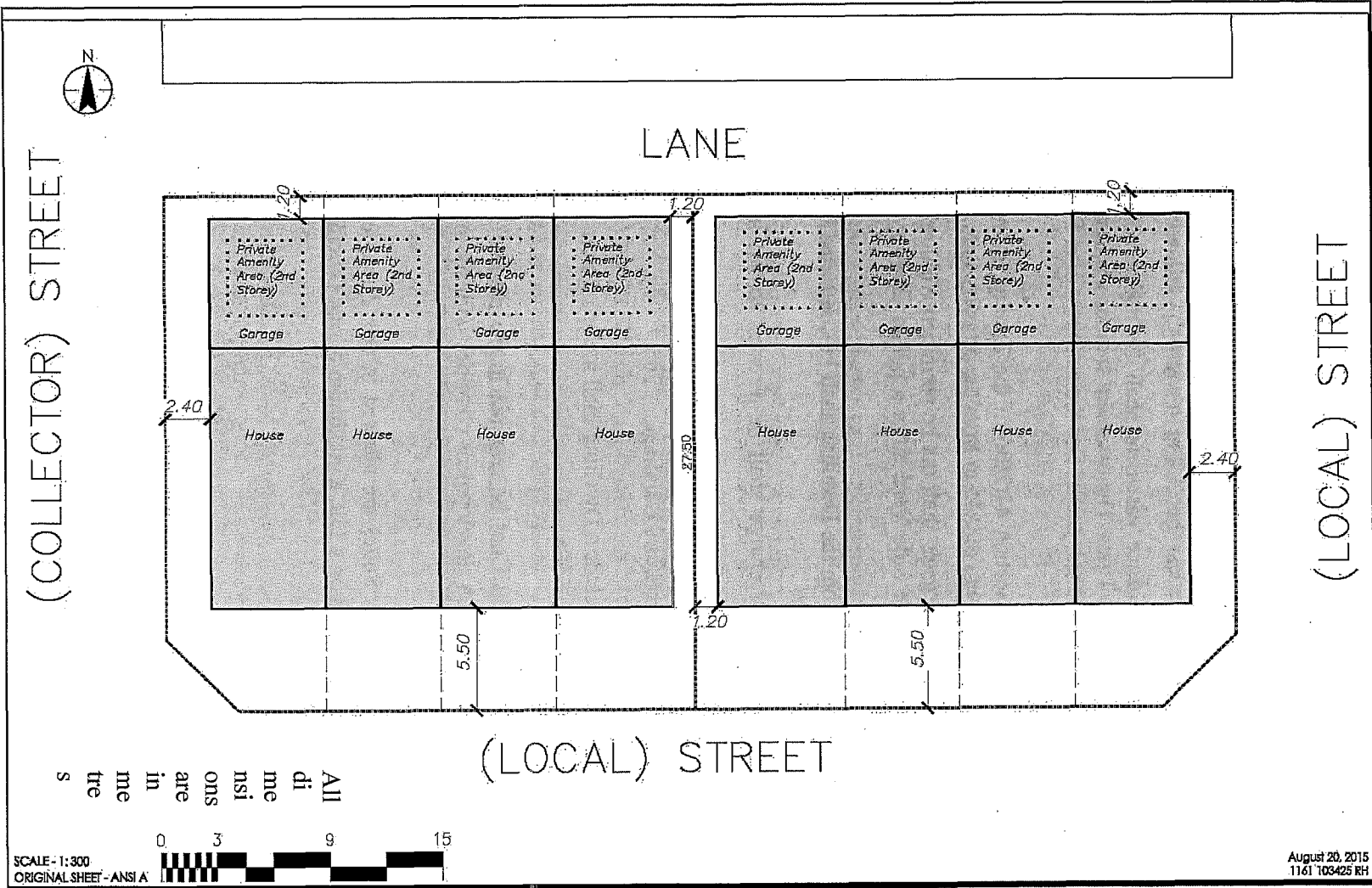
Figure 1. Minimum Setbacks – Row Housing in Area A (Example)
