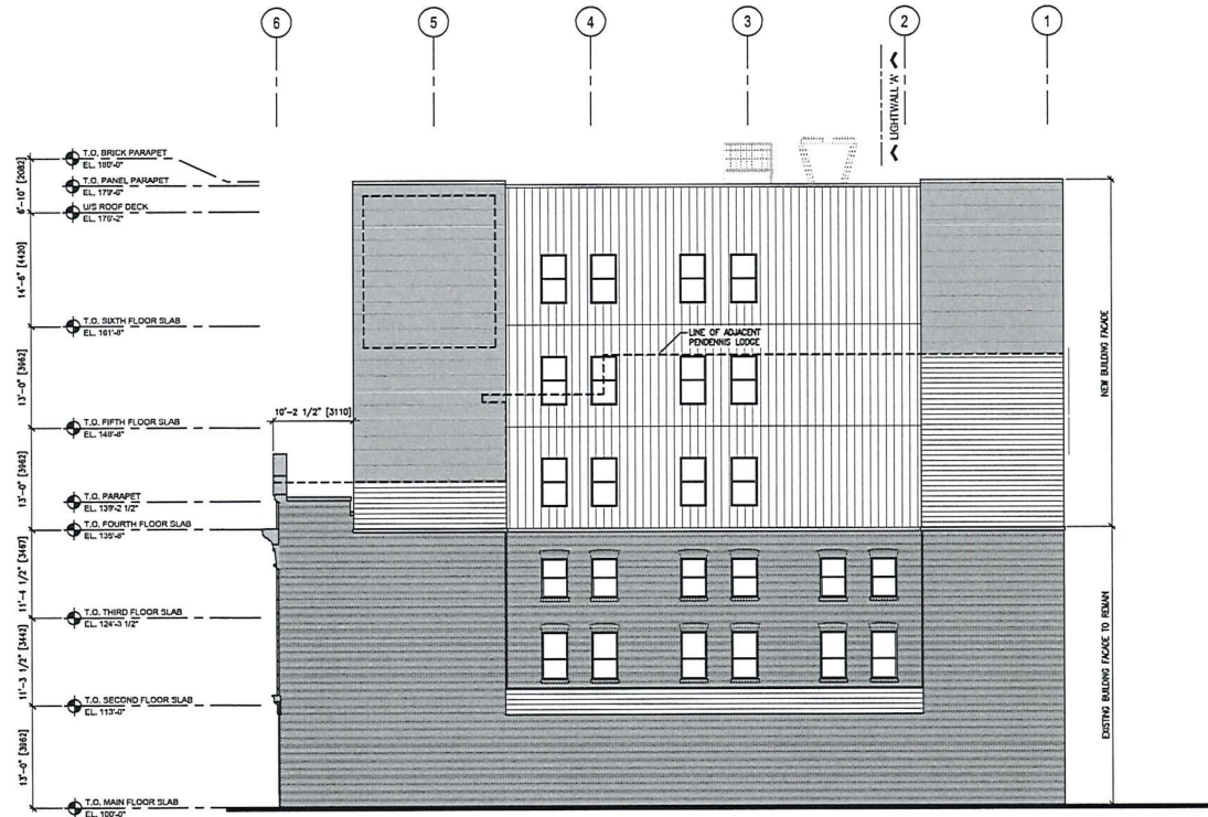
EAST ELEVATION 1/8"=1'-0"
