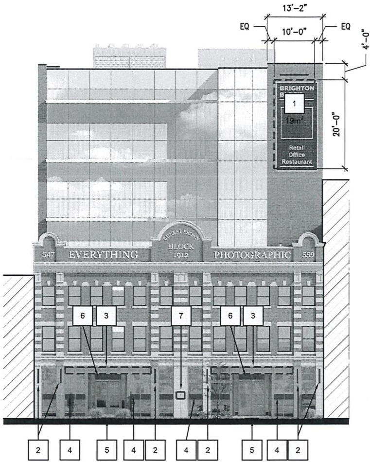
SOUTH ELEVATION
