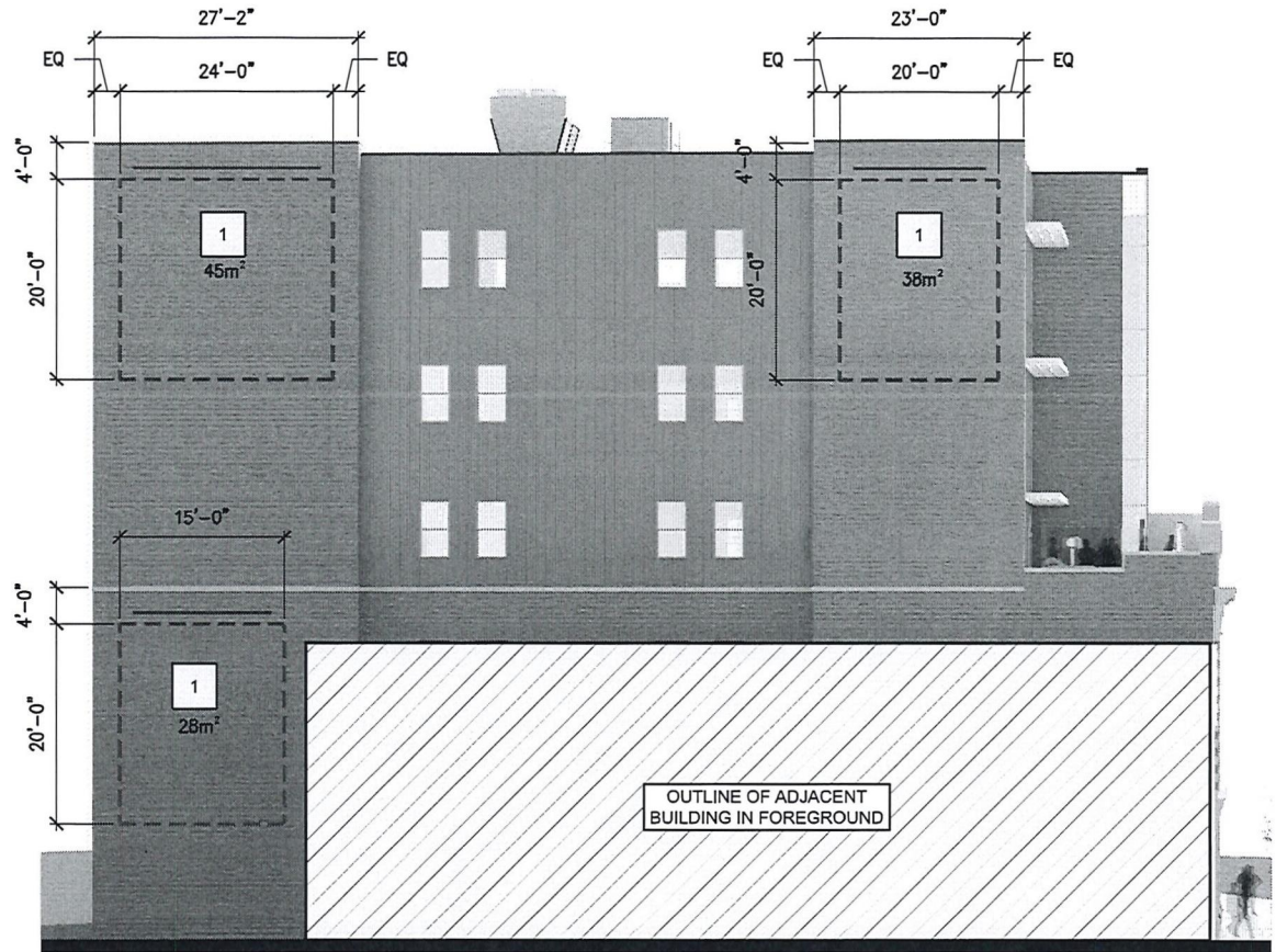
WEST ELEVATION
