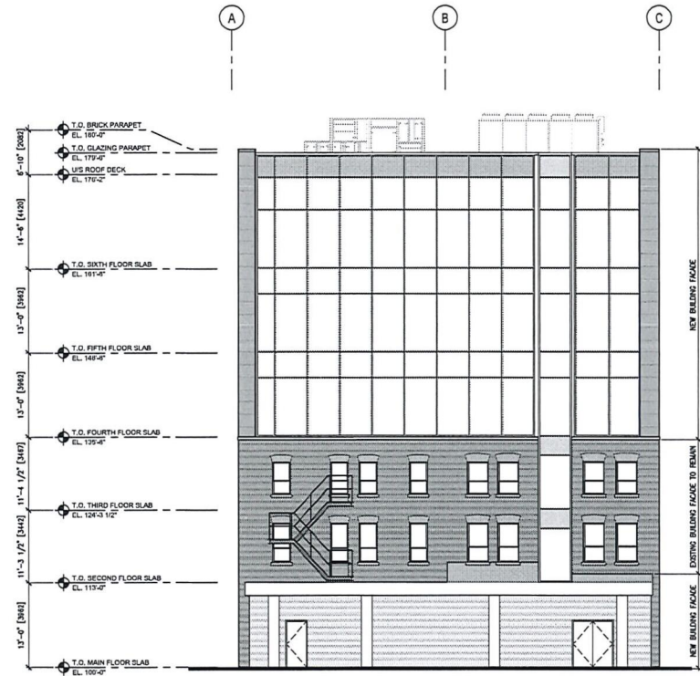
NORTH ELEVATION 1/8"=1'-0"
