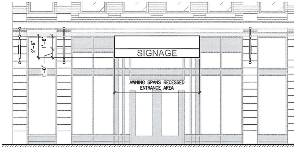
ELEVATION - OPTION 1
