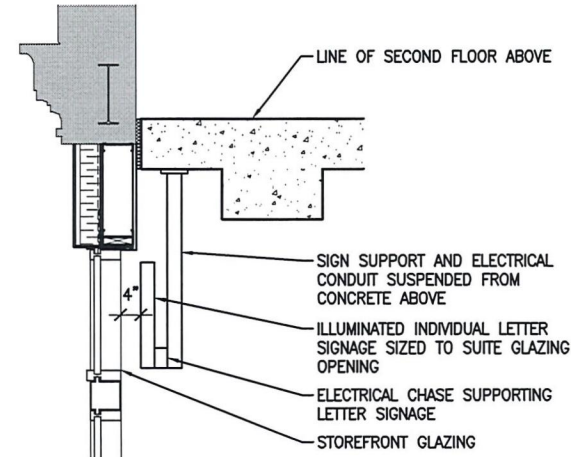
LETTER SIGNAGE SECTION
