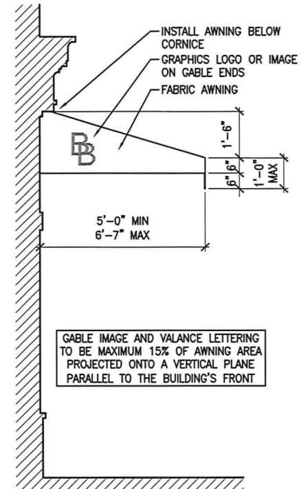
RETRACTABLE AWNING SIDE ELEVATION
