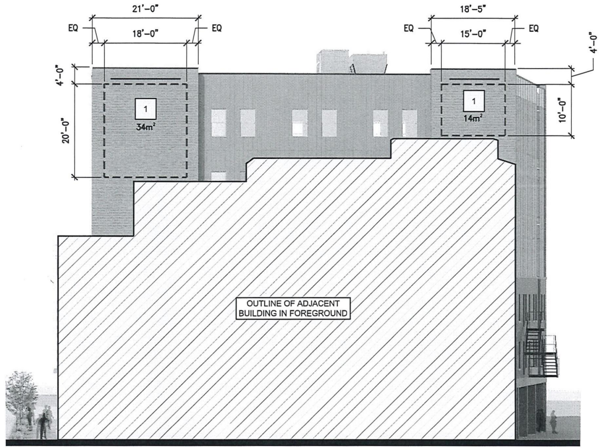
EAST ELEVATION
