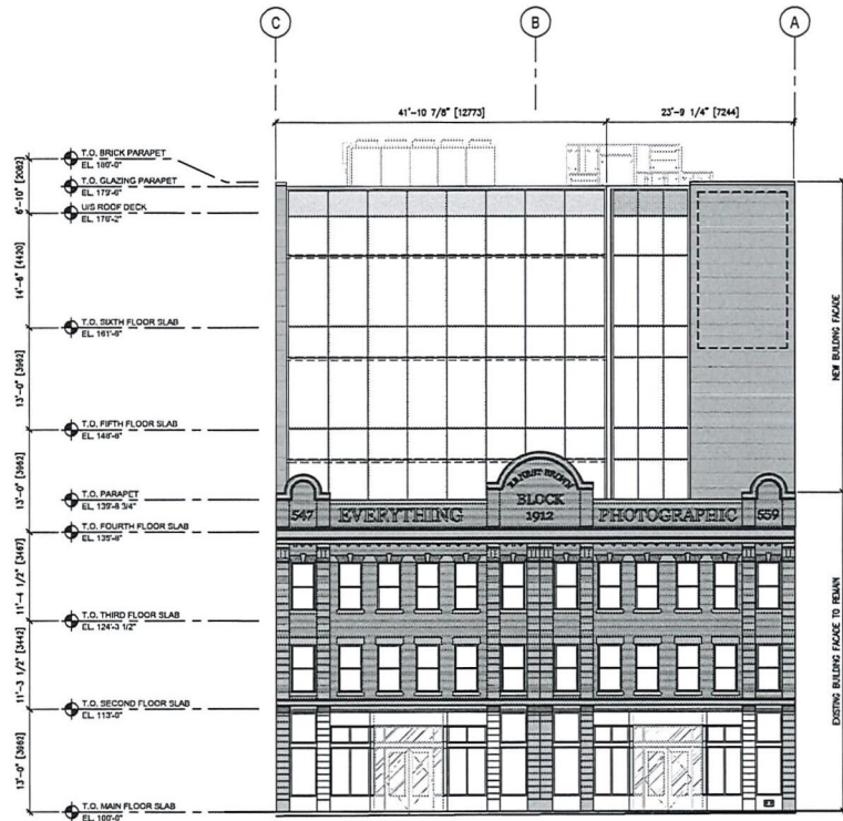
SOUTH ELEVATION 1/8"=1'-0"
