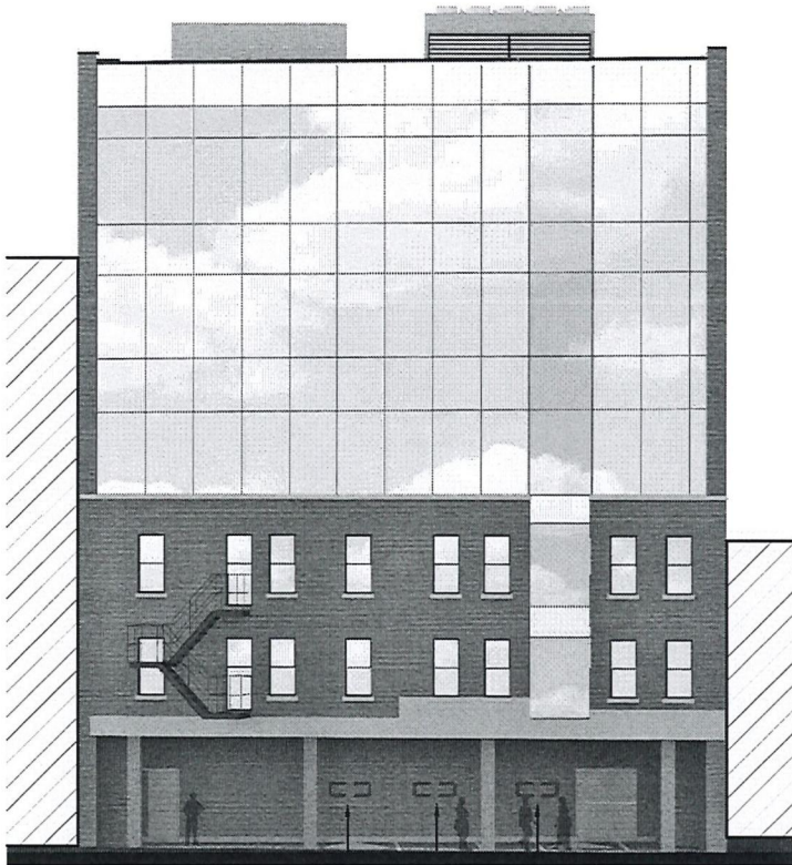
NORTH ELEVATION
