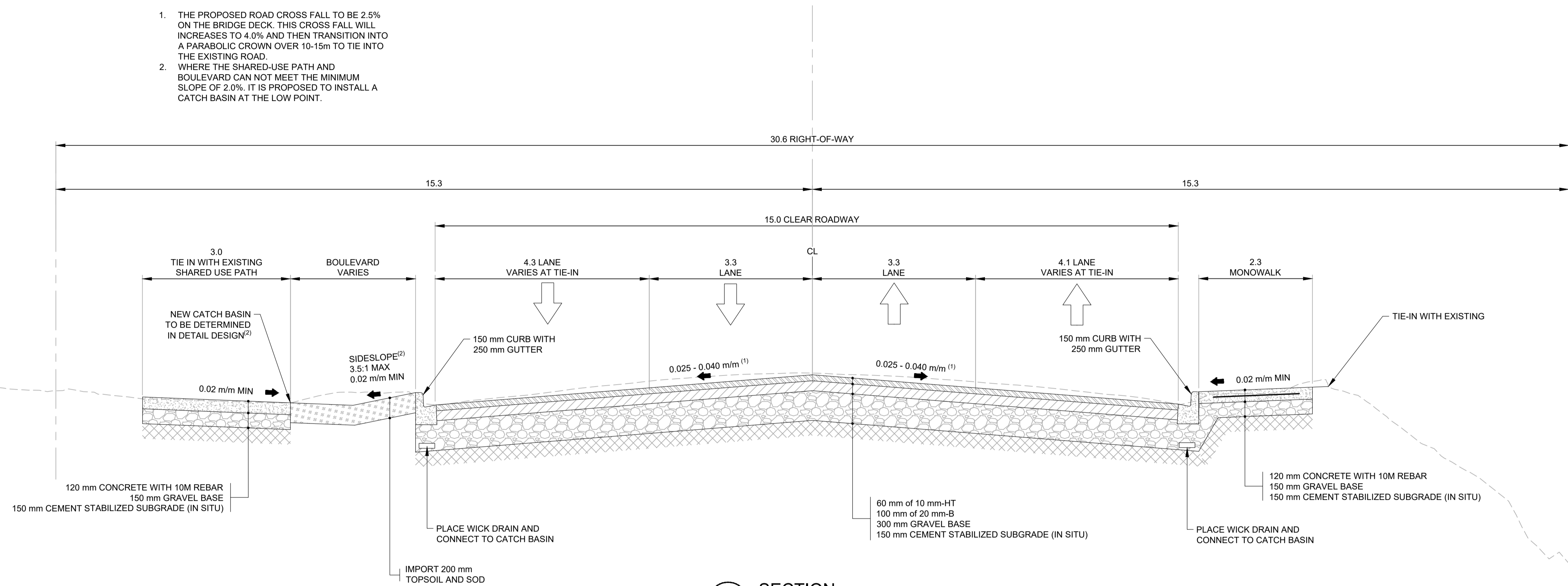
1 SECTION D02 TYPICAL CROSS SECTION FOR RECONSTRUCTION OF 131 STREET 1:50 H 1:25 V
