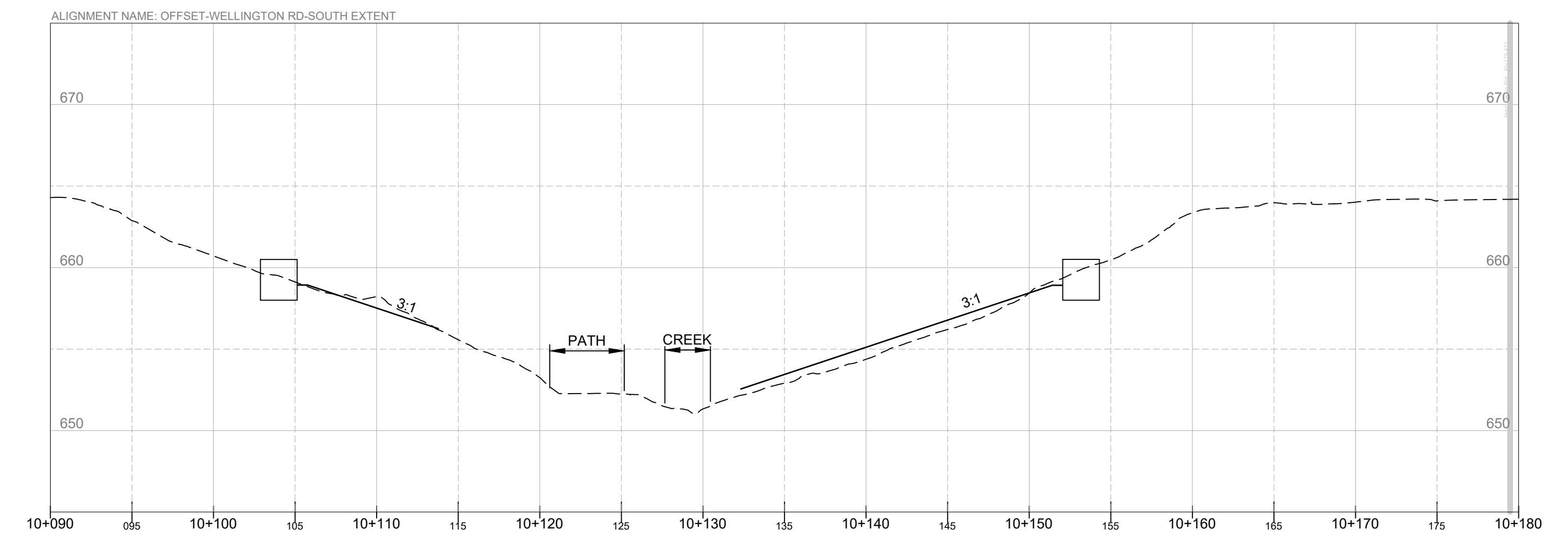
Offset-Wellington Rd-South Extent SCALE 1:250
