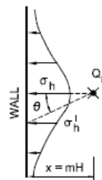
SECTION a-a PRESSURES FROM POINT LOAD Q_p (BOUSSINESQ EQUATION MODIFIED BY EXPERIMENT)
