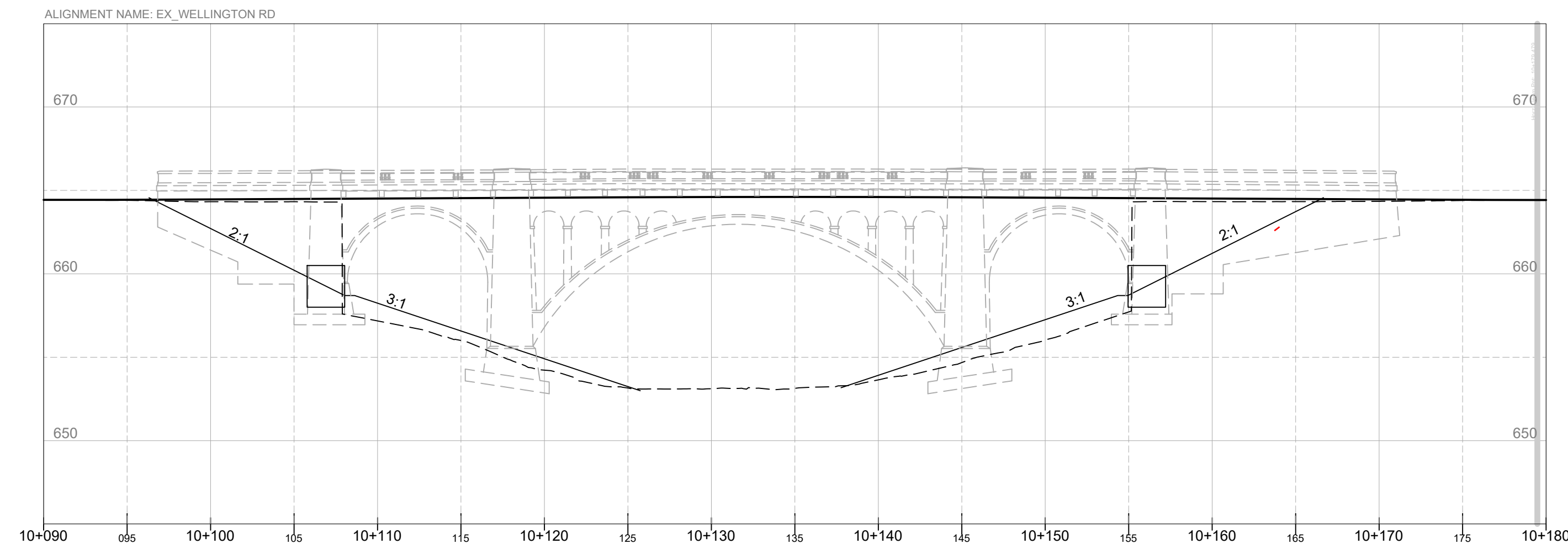
Ex_Wellington Rd SCALE 1:250
