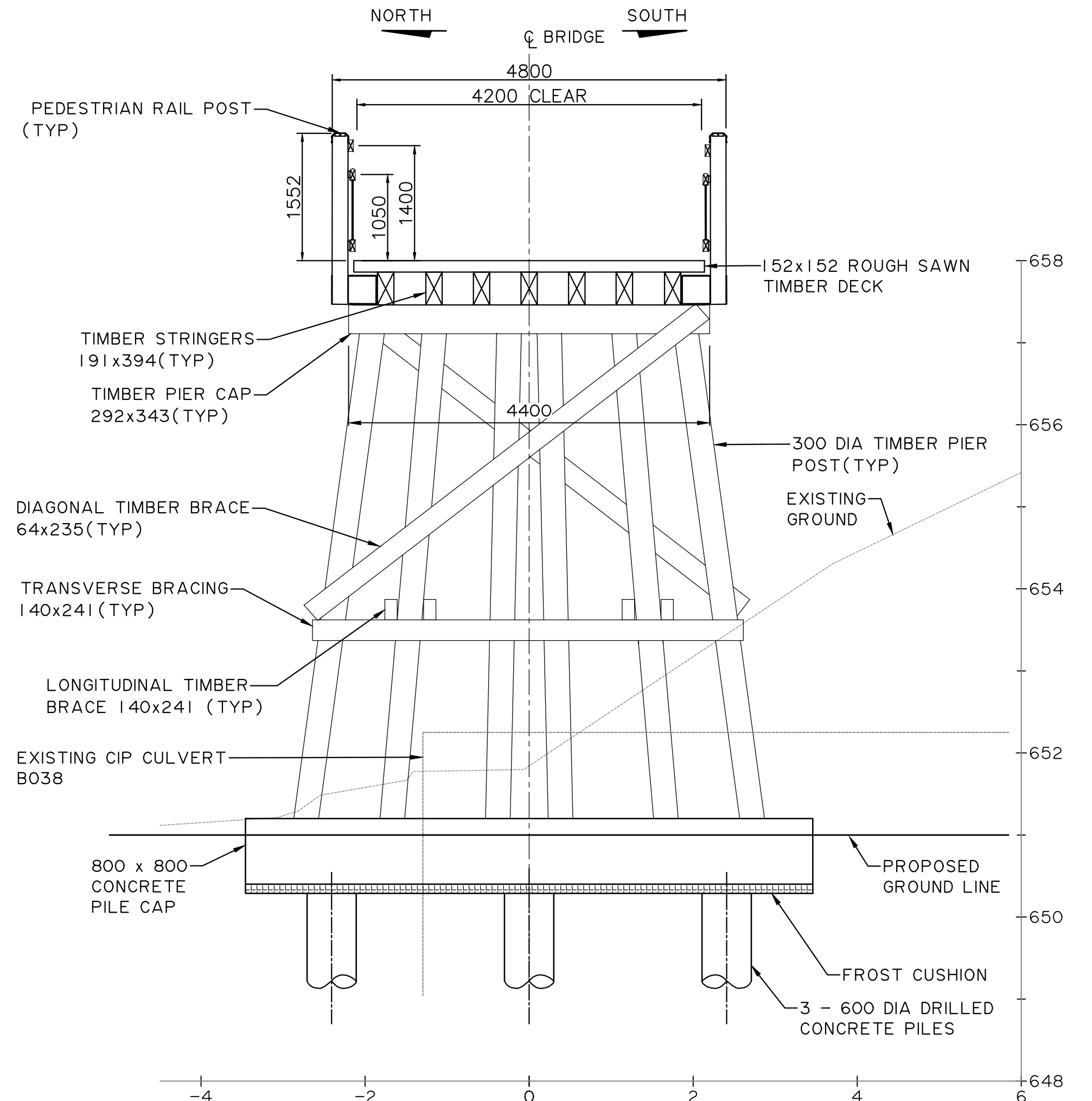
SECTION A PIER 3 1:50
