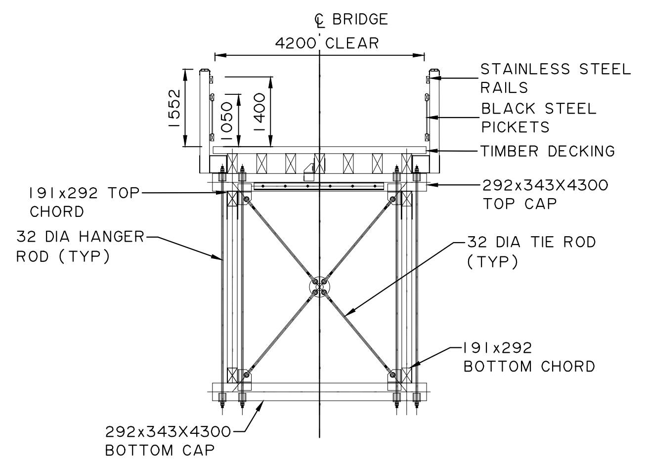
SECTION B PIER 5 1:75
