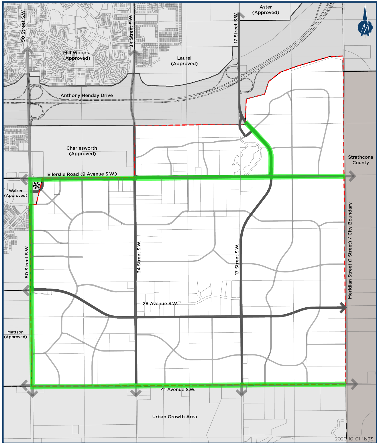
Figure 9 Transportation Network
