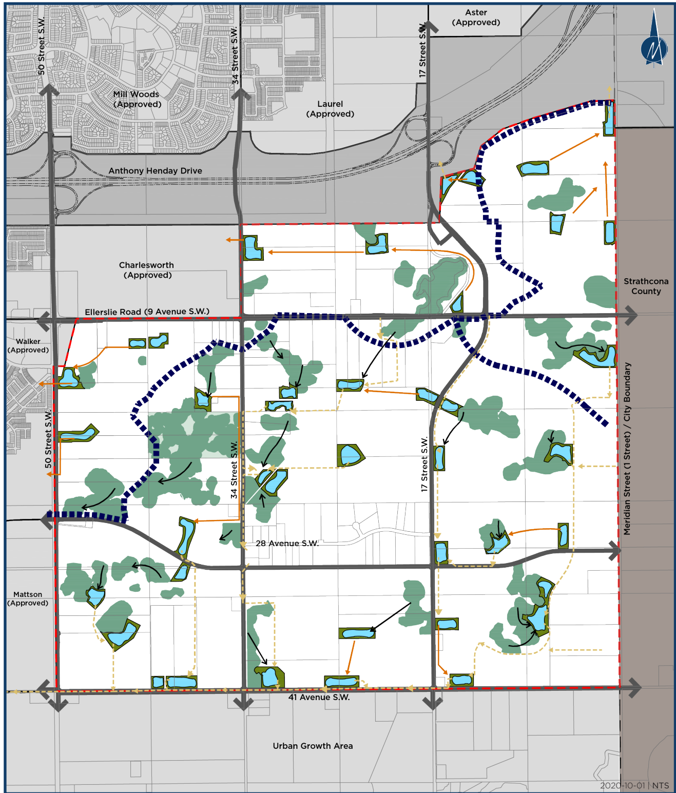
Figure 12 Stormwater Servicing
