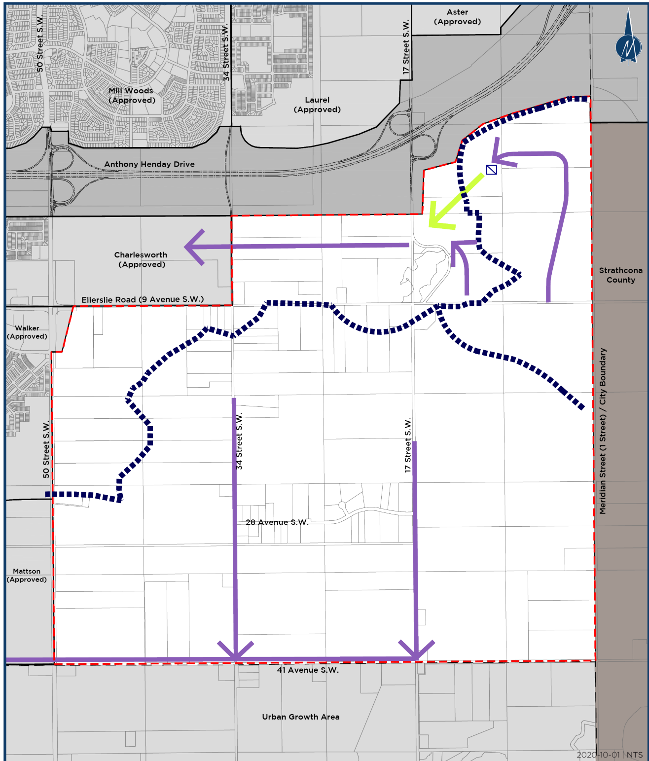
Figure 11 Sanitary Servicing
